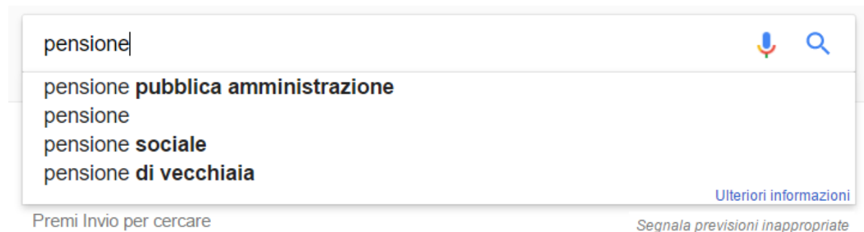
Fig. 4.4: Google suggest
